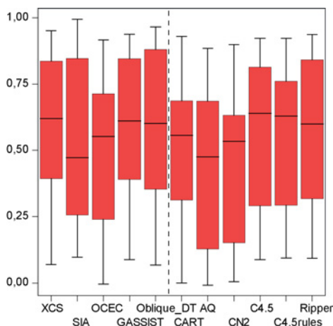
Fig. 8. Box plot representation of the kappa results for the selected GBML and non-evolutionary algorithms.
