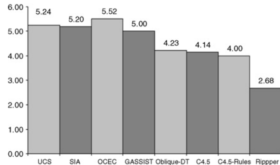
Fig. 15. Ranking computed for the selected GBML and non-evolutionary algorithms in imbalanced data sets.
