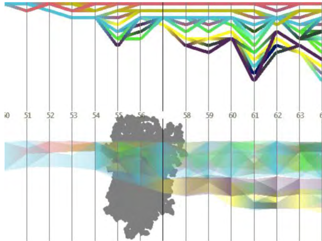
Fig 17. Temporal development of cavities in a bacteriorhodopsin monomer (for the simulation and the time steps also used in Figure 16); upper diagram: topology graph showing splits and merges of cavities; lower diagram: penetration graph depicting the cavities' location along a user-defined axis. The image is based on Refs. (Lindow et al., 2012a; Lindow et al., 2013)
